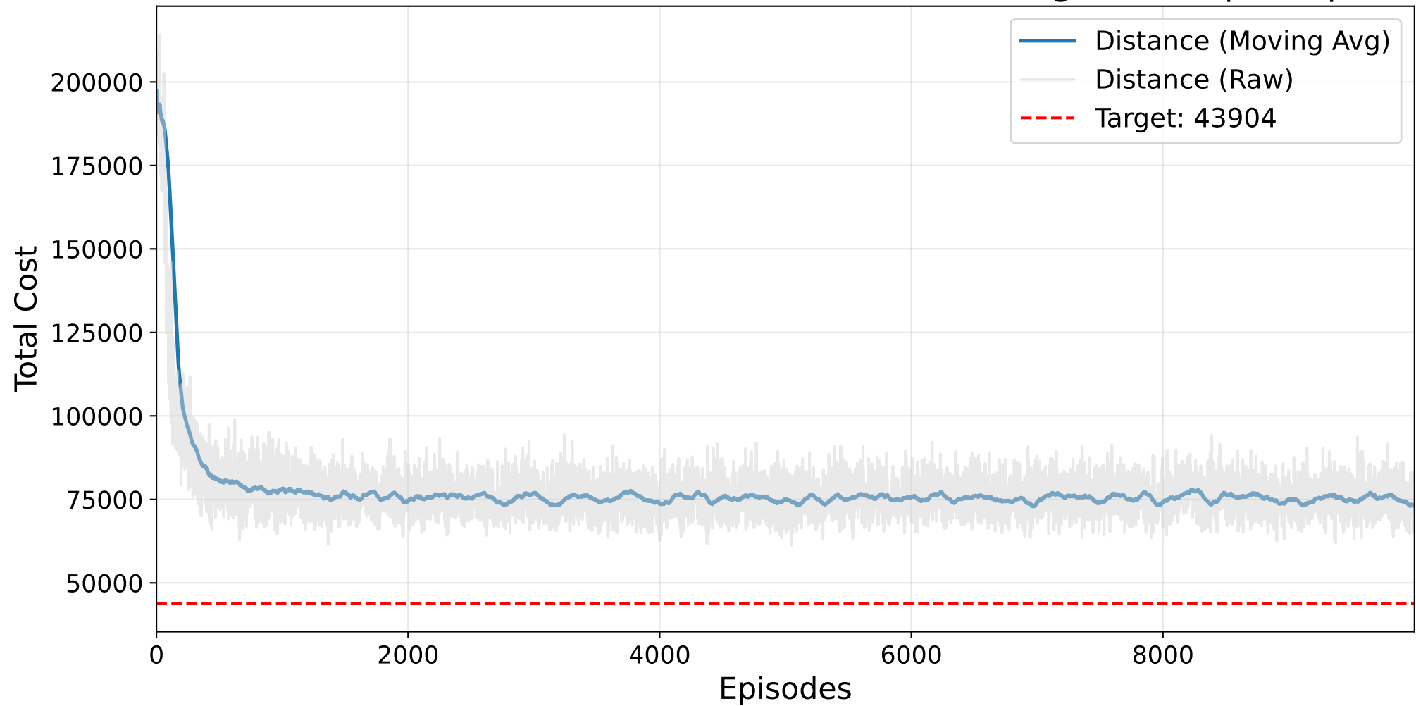
Final HYPERBAND GP Masked AutoRL-SOP Training - kro124p.3.sop
